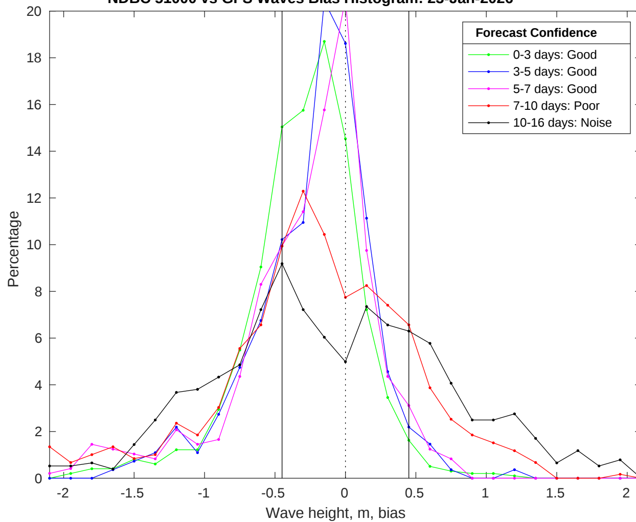
NDBC 51000 vs GFS Waves Bias Histogram: 23-Jan-2026
