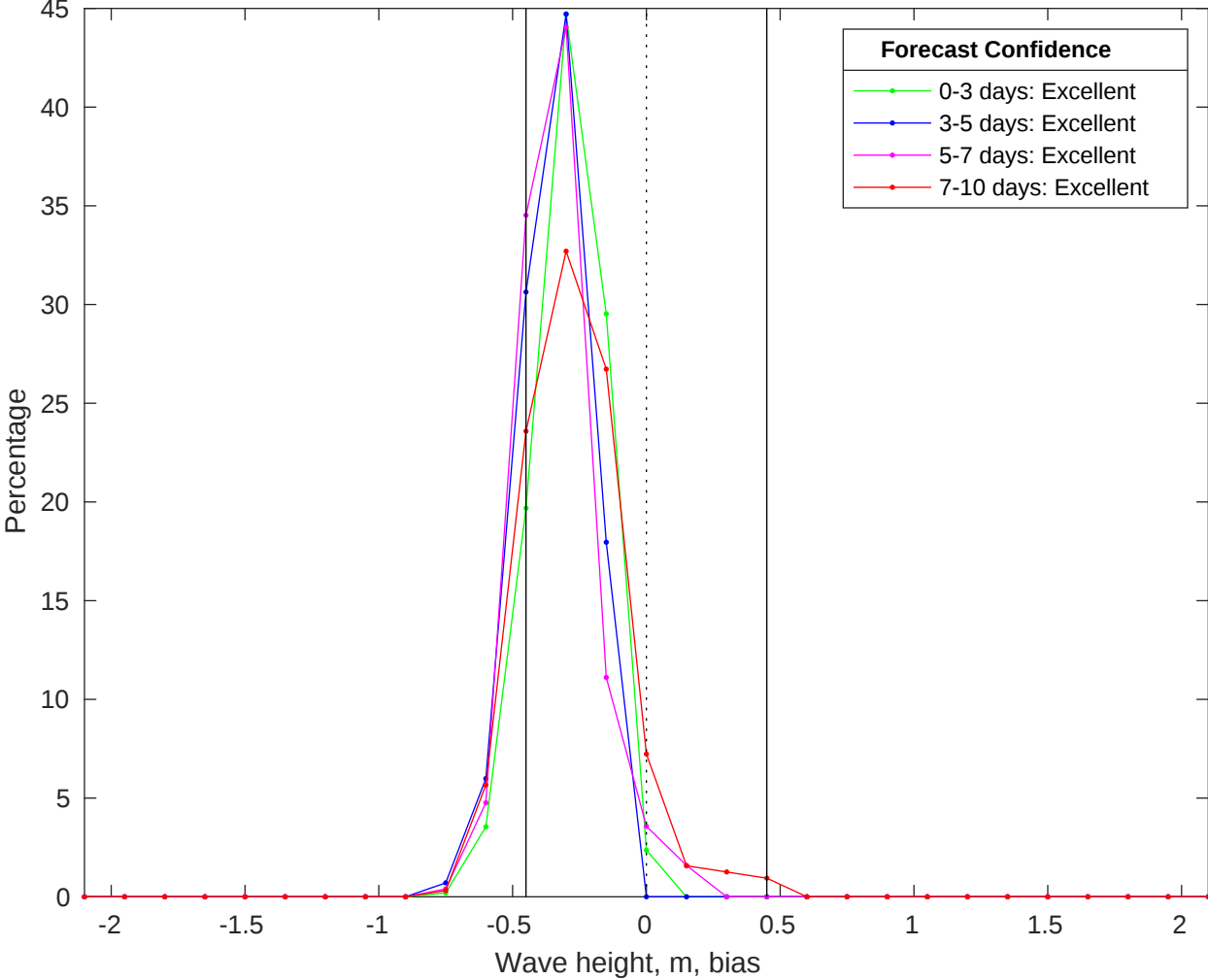
NDBC 51209 vs CMEMS Waves Bias Histogram: 23-Jan-2026
