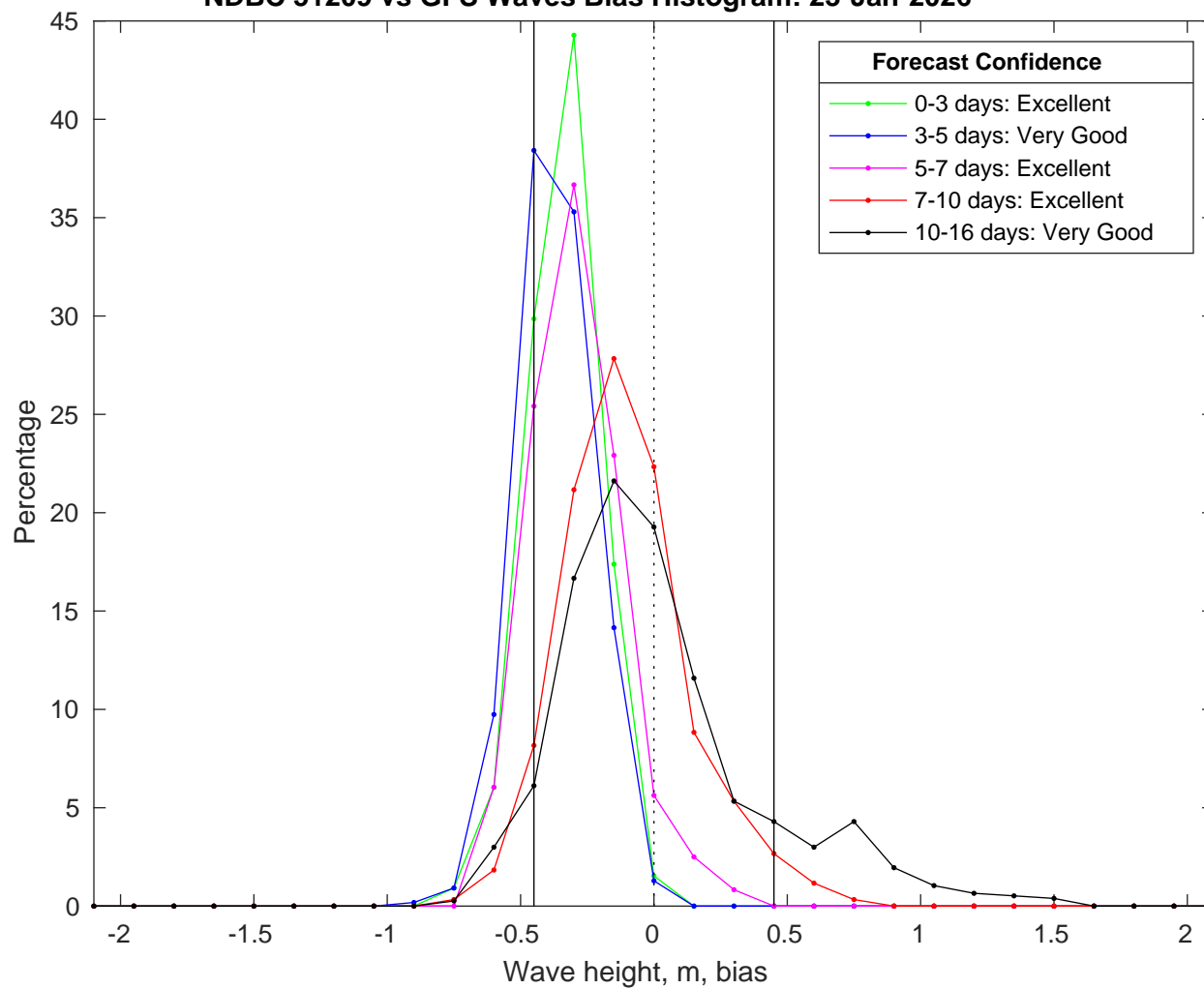
NDBC 51209 vs GFS Waves Bias Histogram: 23-Jan-2026
