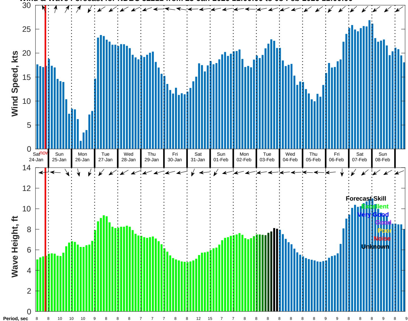
Wind & Wave Forecast for NDBC 52211 from 23-Jan-2026 11:00:00 to 08-Feb-2026 11:00:00
