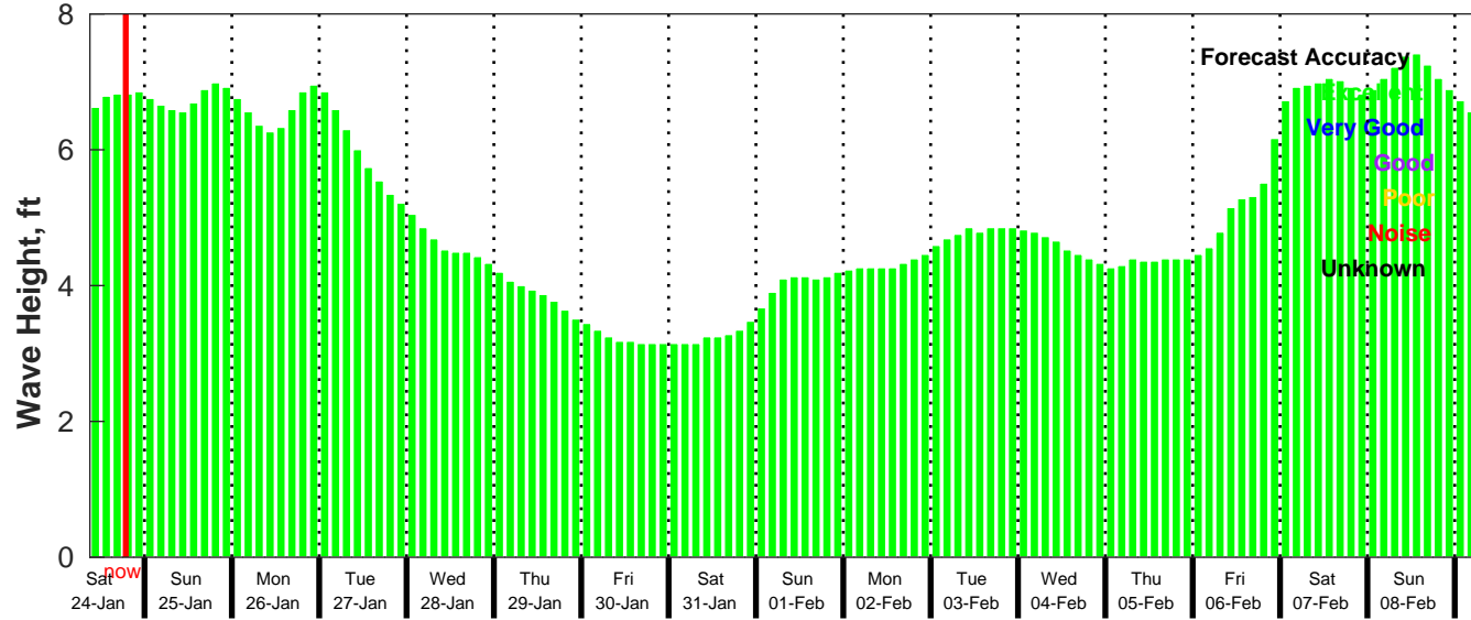
GFS Wave Forecast for NDBC 52212 from 23-Jan-2026 09:00:00 to 08-Feb-2026 09:00:00
