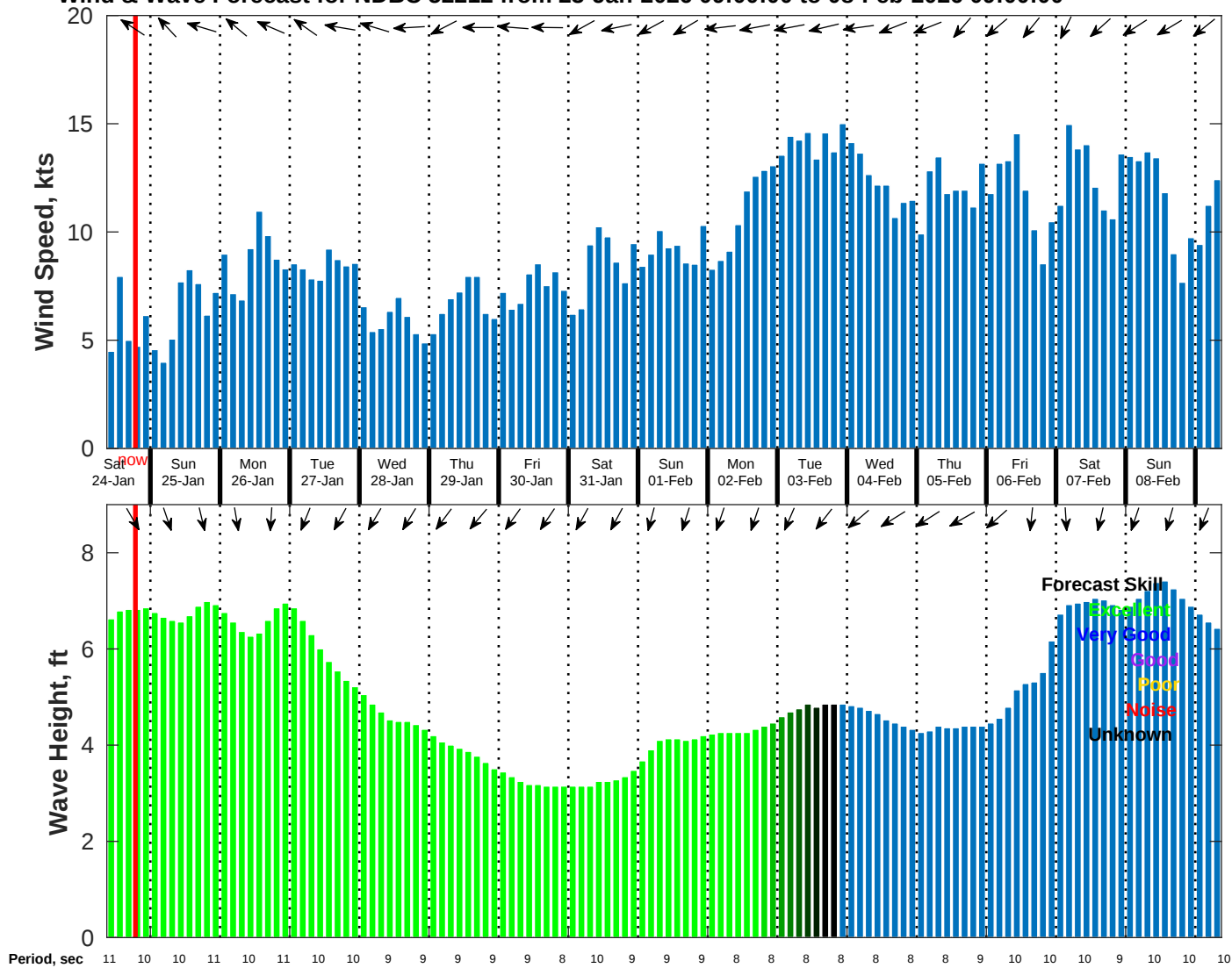
Wind & Wave Forecast for NDBC 52212 from 23-Jan-2026 09:00:00 to 08-Feb-2026 09:00:00
