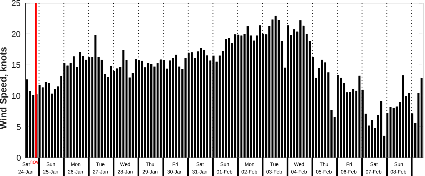
GFS Wind Speed Forecast for NDBC 52213 from 23-Jan-2026 11:00:00 to 08-Feb-2026 11:00:00
