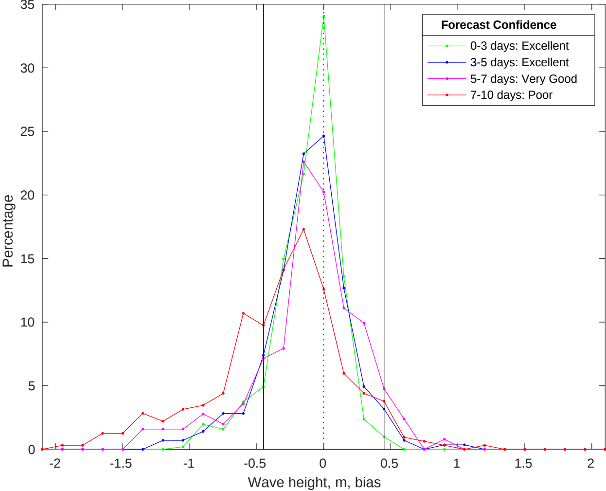
NDBC 41004 vs CMEMS Waves Bias Histogram: 24-Jan-2026
