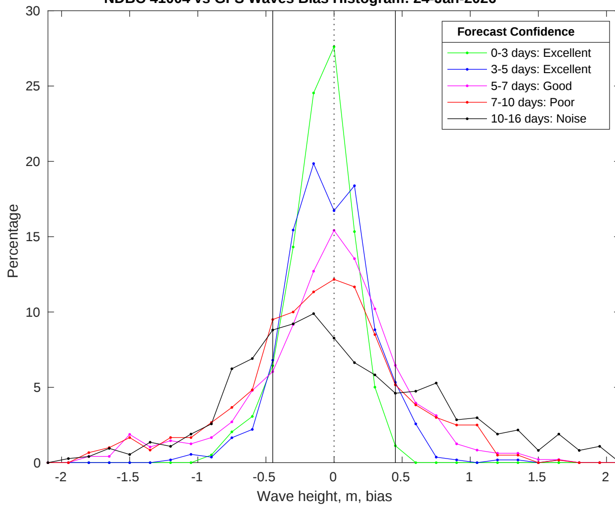
NDBC 41004 vs GFS Waves Bias Histogram: 24-Jan-2026
