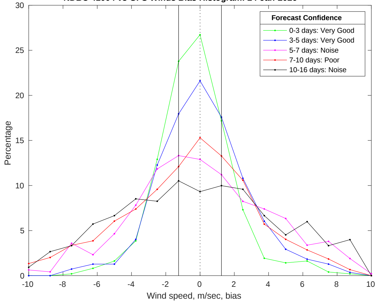
NDBC 41004 vs GFS Winds Bias Histogram: 24-Jan-2026
