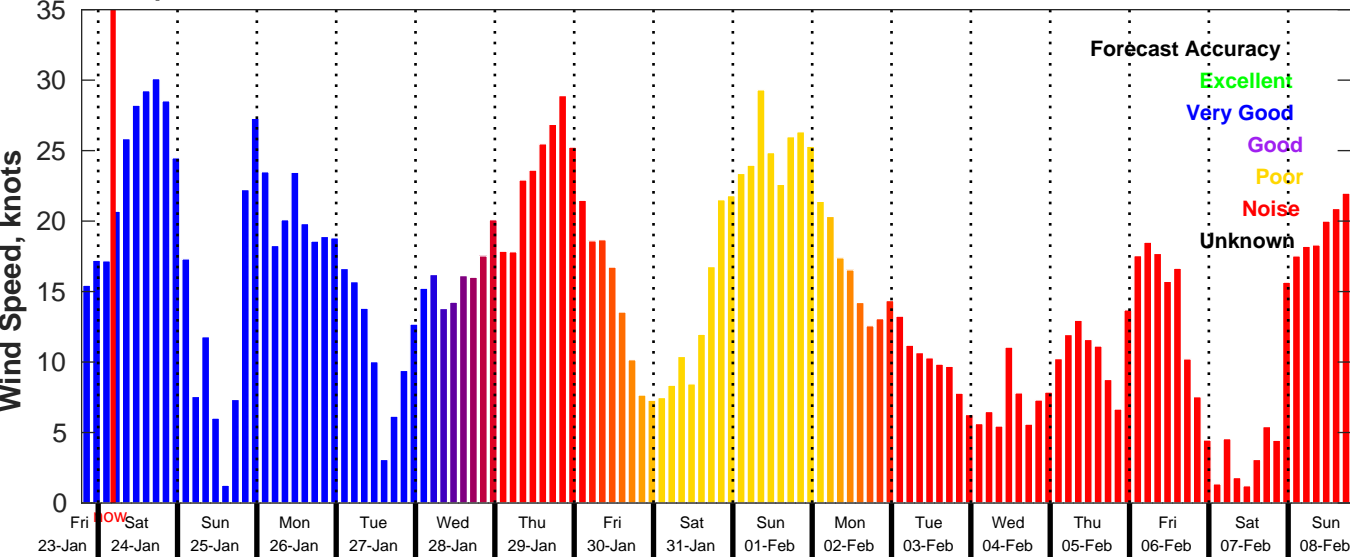
GFS Wind Speed Forecast for NDBC 41004 from 23-Jan-2026 19:00:00 to 08-Feb-2026 19:00:00
