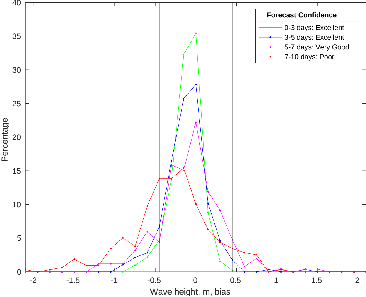
NDBC 41013 vs CMEMS Waves Bias Histogram: 24-Jan-2026
