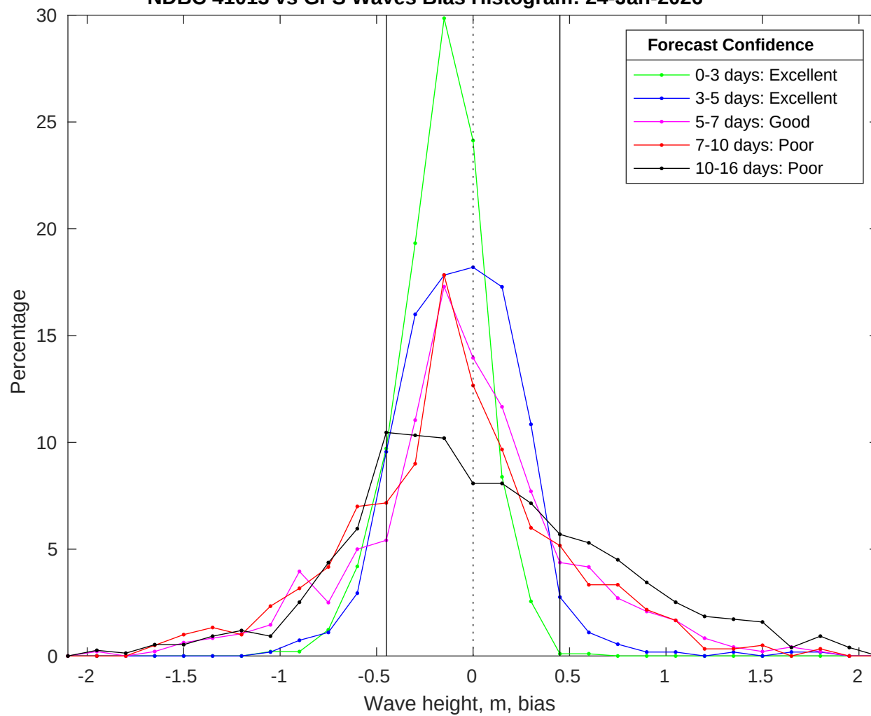
NDBC 41013 vs GFS Waves Bias Histogram: 24-Jan-2026
