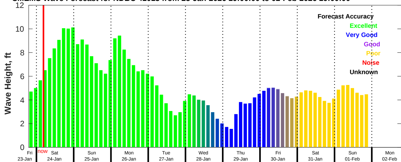
CMEMS Wave Forecast for NDBC 41013 from 23-Jan-2026 19:00:00 to 02-Feb-2026 19:00:00
