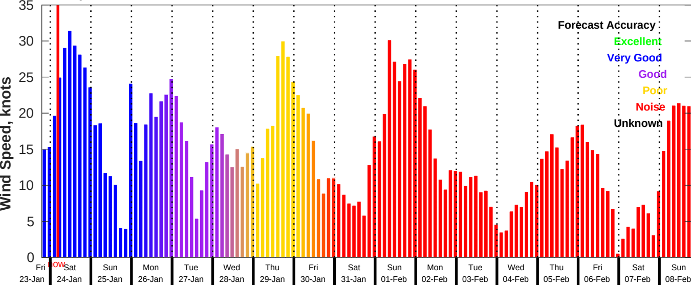
GFS Wind Speed Forecast for NDBC 41013 from 23-Jan-2026 19:00:00 to 08-Feb-2026 19:00:00
