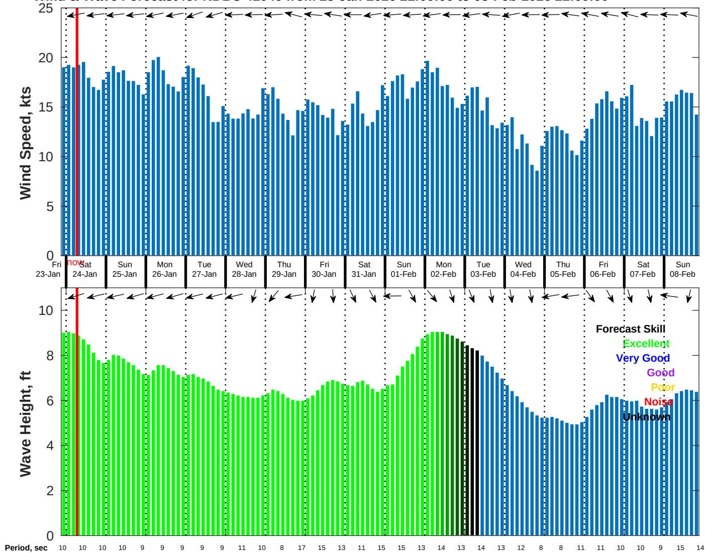
Wind & Wave Forecast for NDBC 41040 from 23-Jan-2026 21:00:00 to 08-Feb-2026 21:00:00
