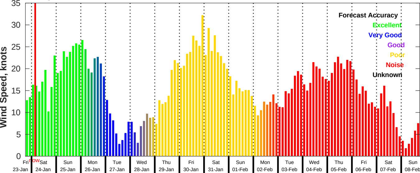
GFS Wind Speed Forecast for NDBC 42019 from 23-Jan-2026 18:00:00 to 08-Feb-2026 18:00:00
