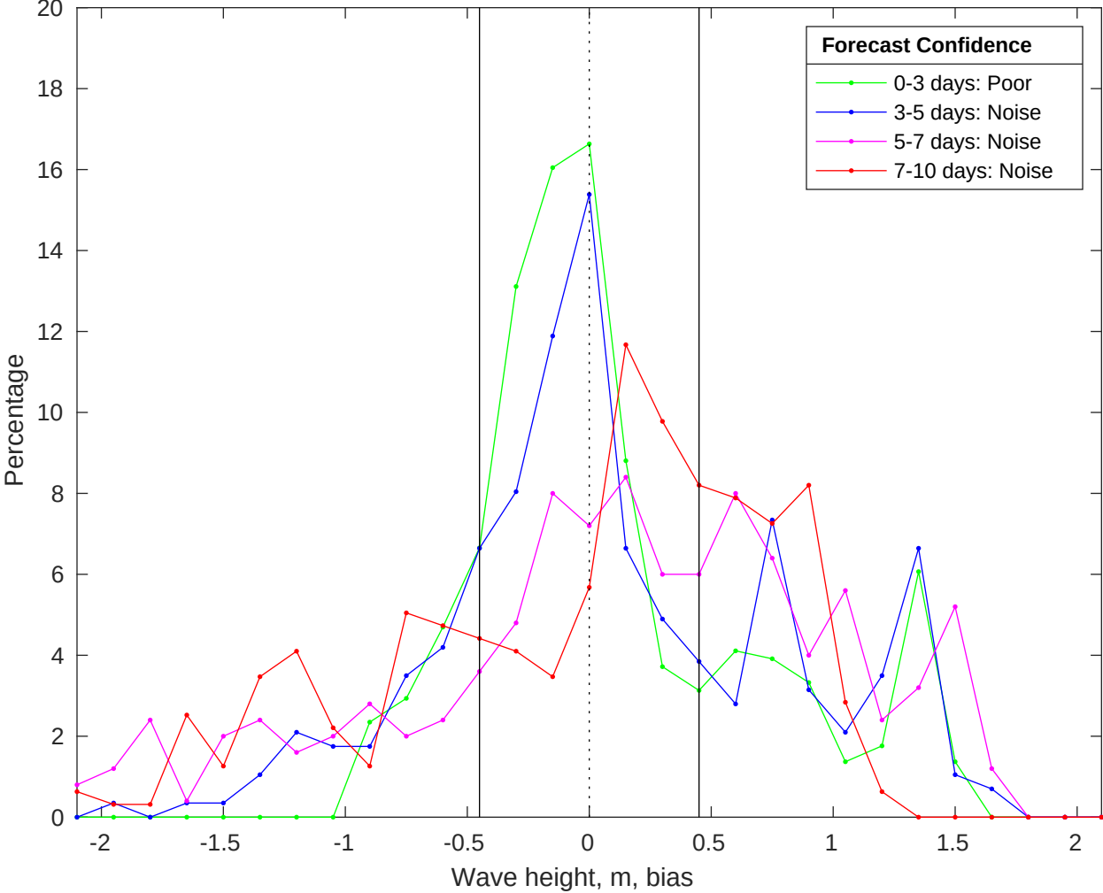
NDBC 42020 vs CMEMS Waves Bias Histogram: 24-Jan-2026
