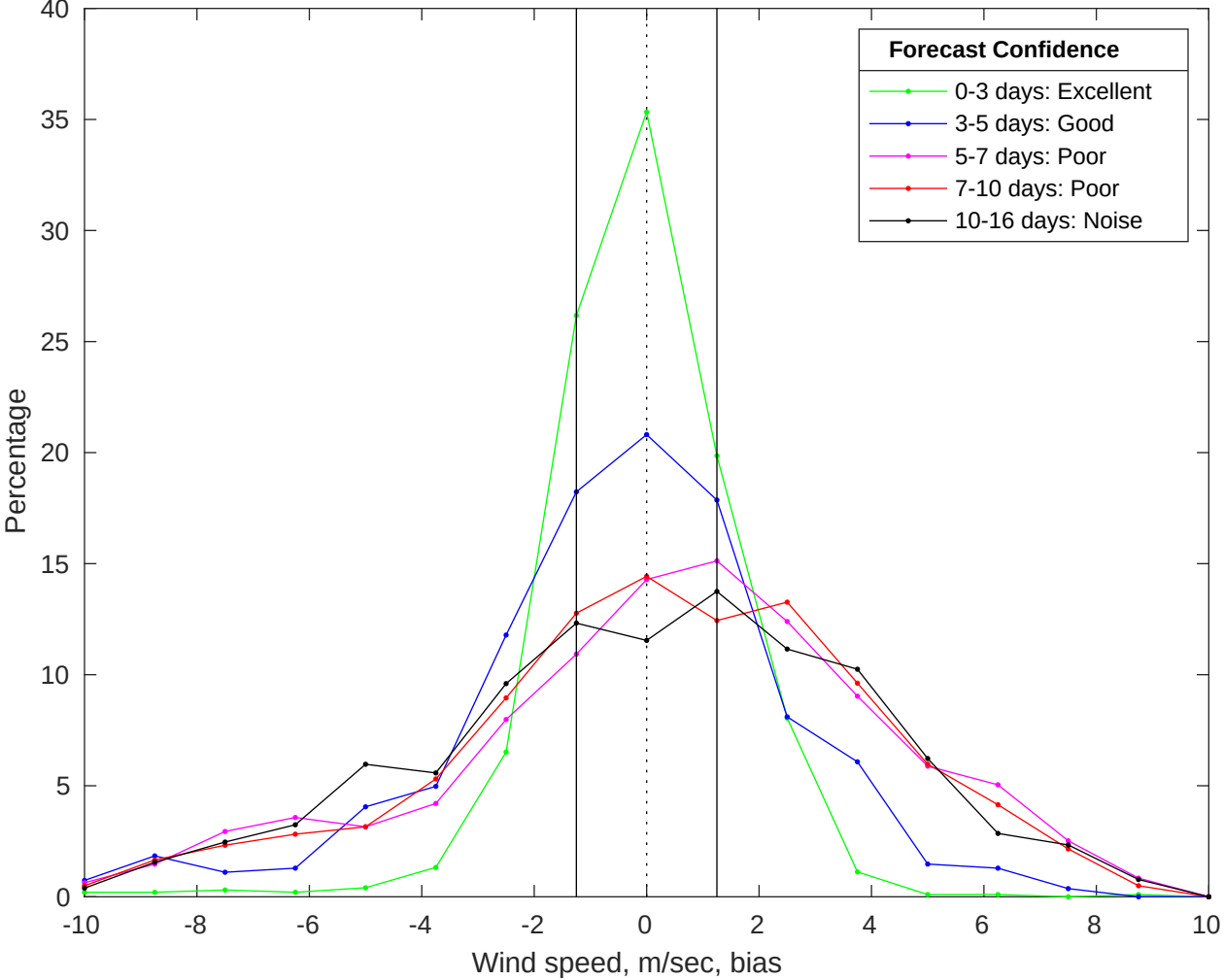
NDBC 42020 vs GFS Winds Bias Histogram: 24-Jan-2026
