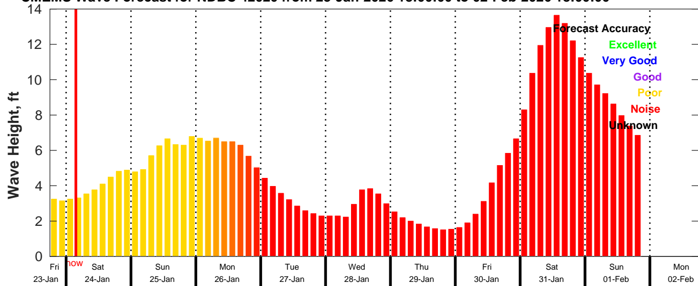
CMEMS Wave Forecast for NDBC 42020 from 23-Jan-2026 18:00:00 to 02-Feb-2026 18:00:00
