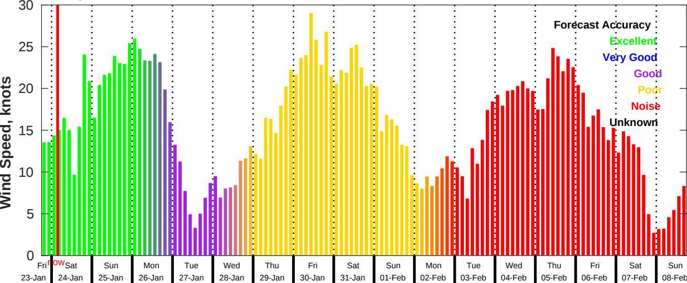
GFS Wind Speed Forecast for NDBC 42020 from 23-Jan-2026 18:00:00 to 08-Feb-2026 18:00:00
