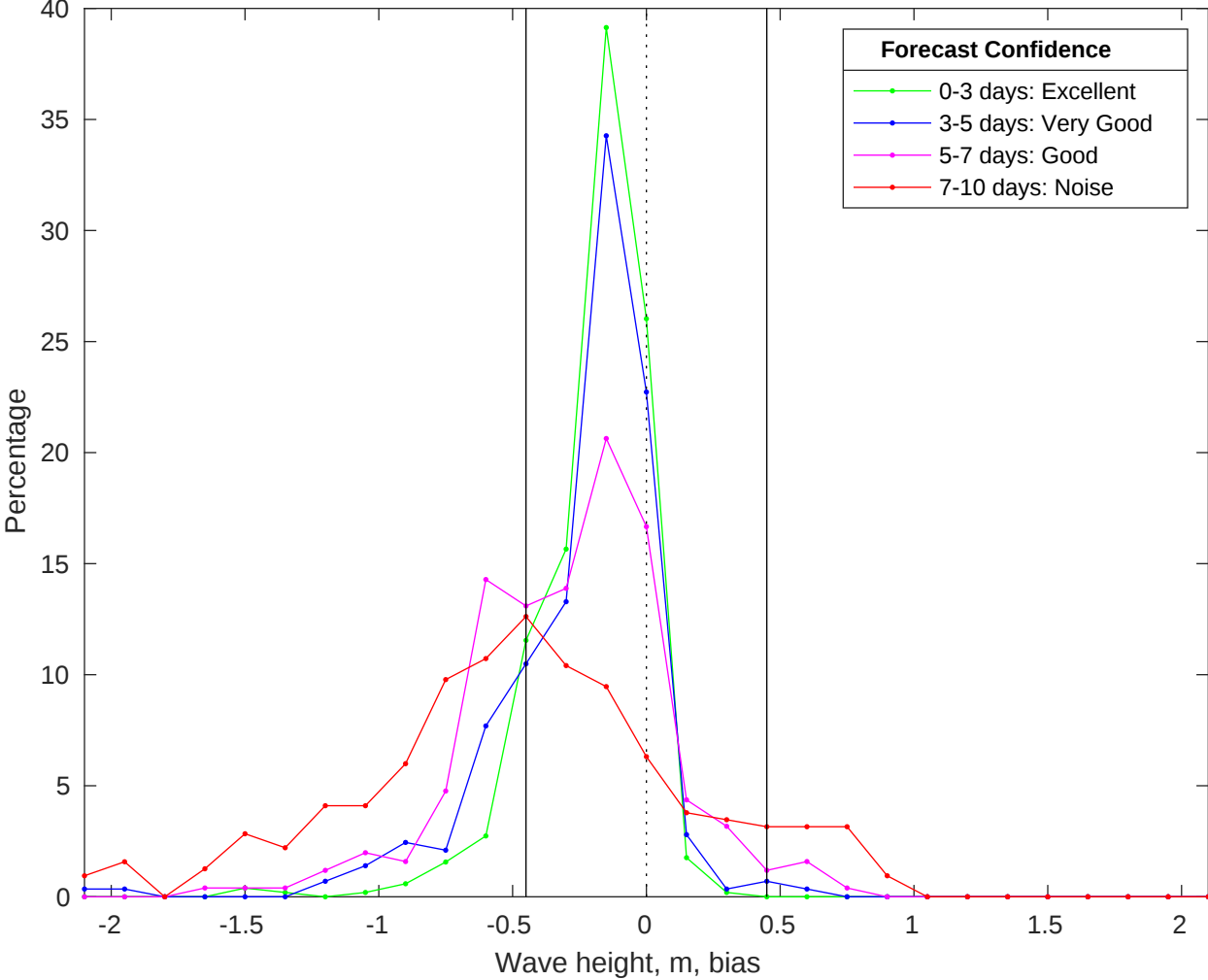
NDBC 42036 vs CMEMS Waves Bias Histogram: 24-Jan-2026
