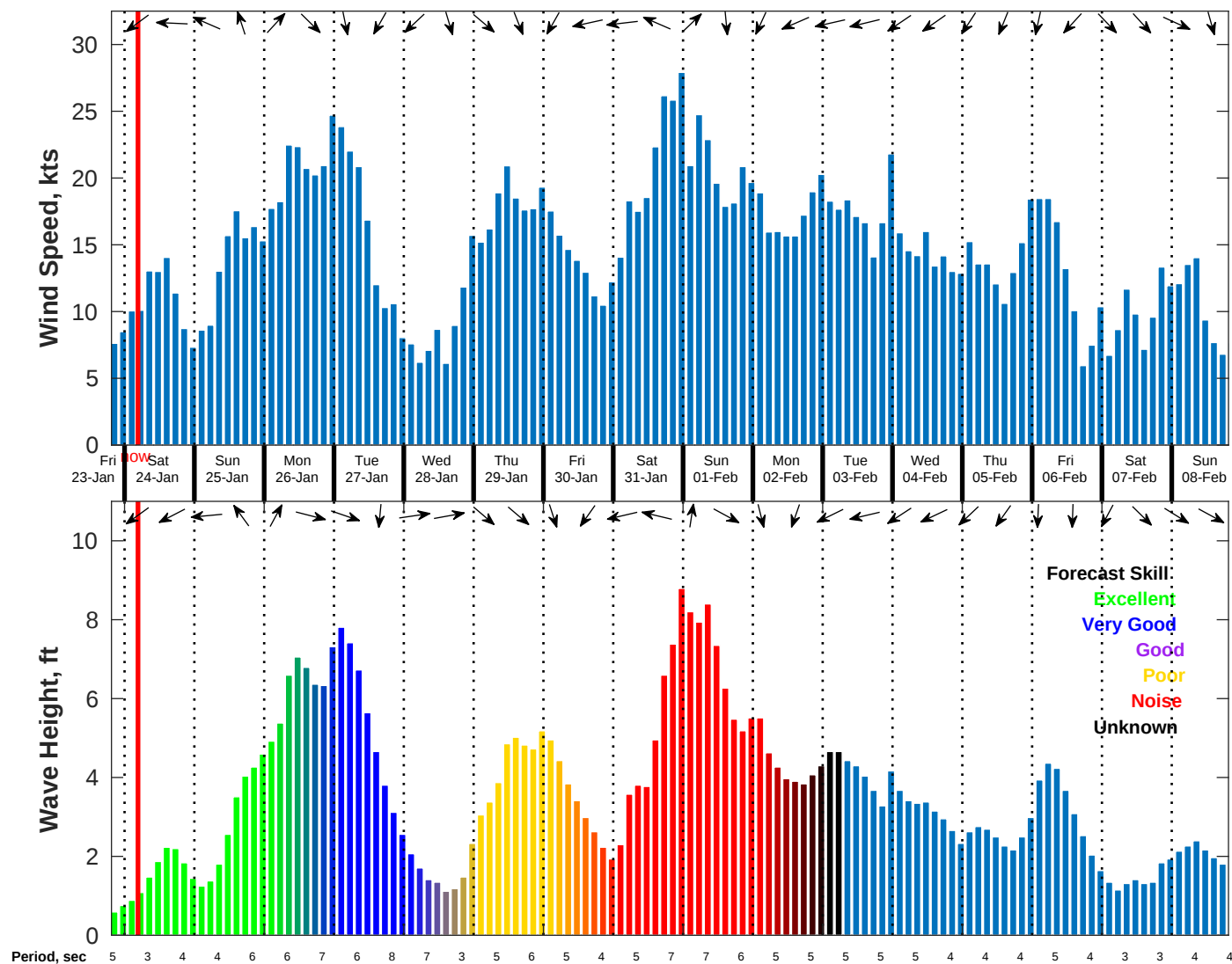
Wind & Wave Forecast for NDBC 42036 from 23-Jan-2026 19:00:00 to 08-Feb-2026 19:00:00
