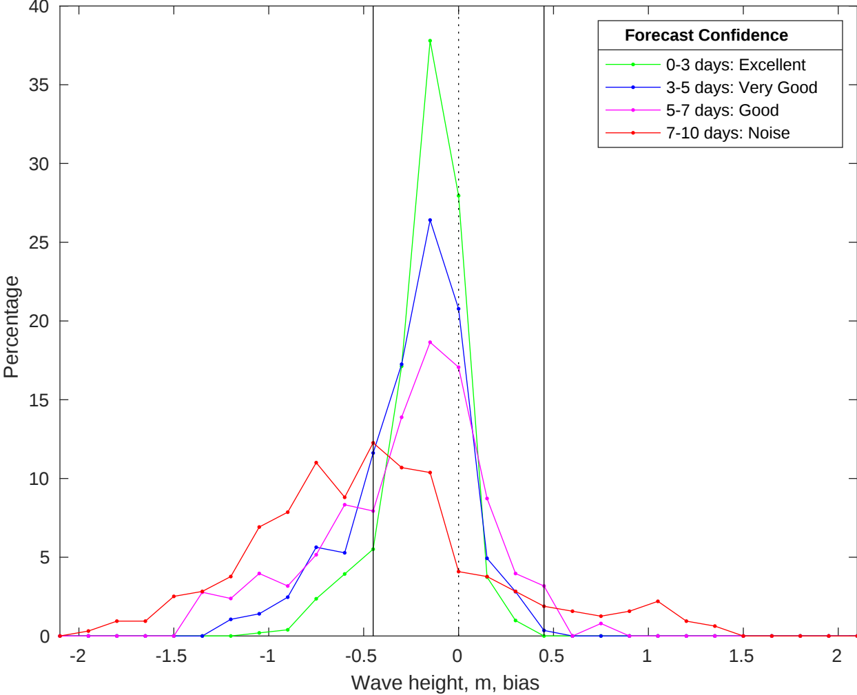
NDBC 42040 vs CMEMS Waves Bias Histogram: 24-Jan-2026
