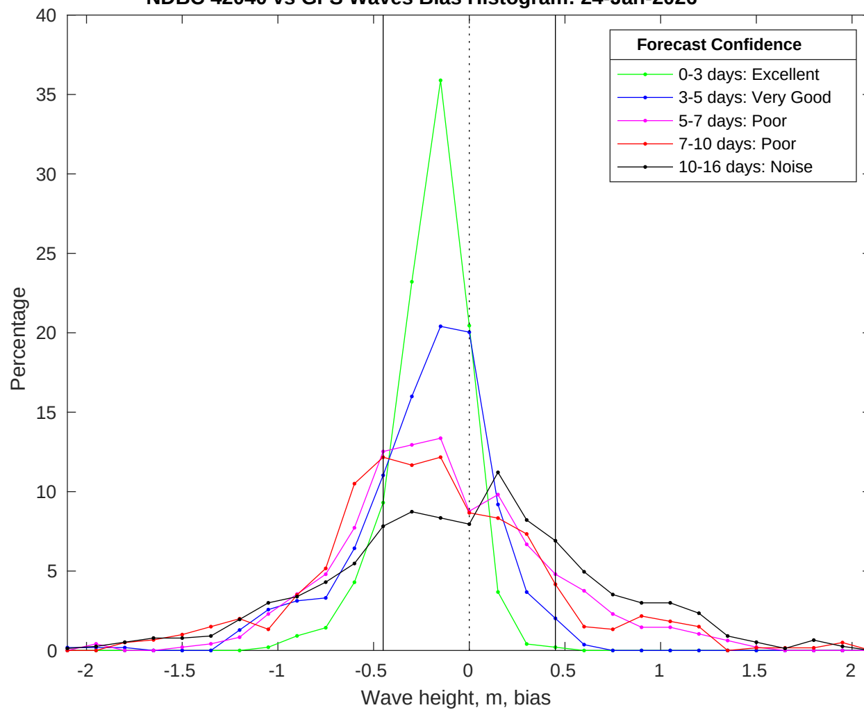
NDBC 42040 vs GFS Waves Bias Histogram: 24-Jan-2026
