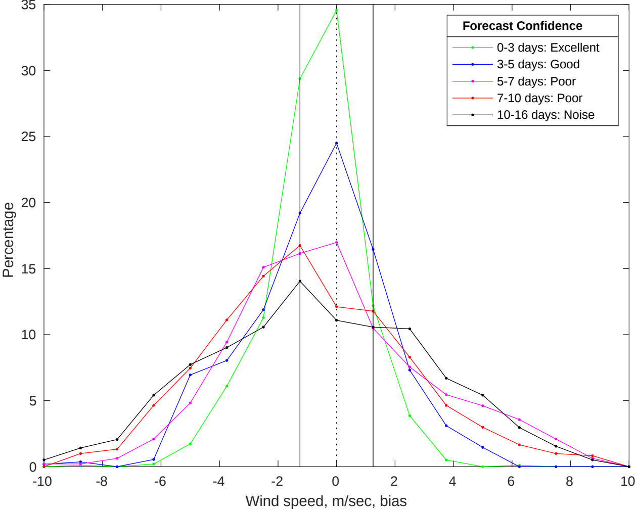
NDBC 42040 vs GFS Winds Bias Histogram: 24-Jan-2026
