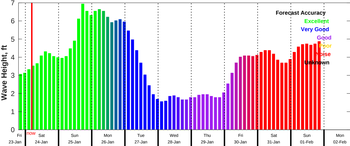
CMEMS Wave Forecast for NDBC 42040 from 23-Jan-2026 19:00:00 to 02-Feb-2026 19:00:00
