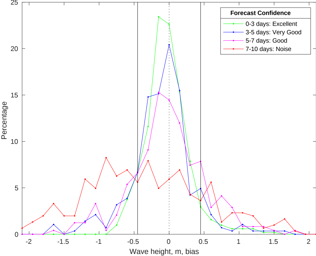
NDBC 44008 vs CMEMS Waves Bias Histogram: 24-Jan-2026
