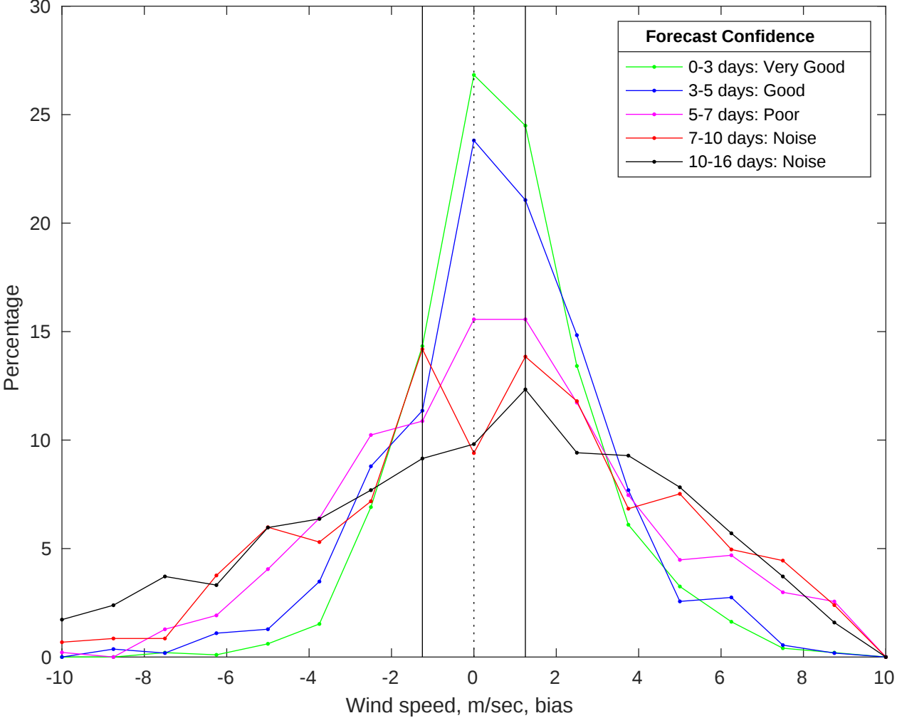
NDBC 44008 vs GFS Winds Bias Histogram: 24-Jan-2026
