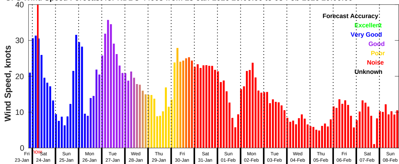
GFS Wind Speed Forecast for NDBC 44008 from 23-Jan-2026 20:00:00 to 08-Feb-2026 20:00:00
