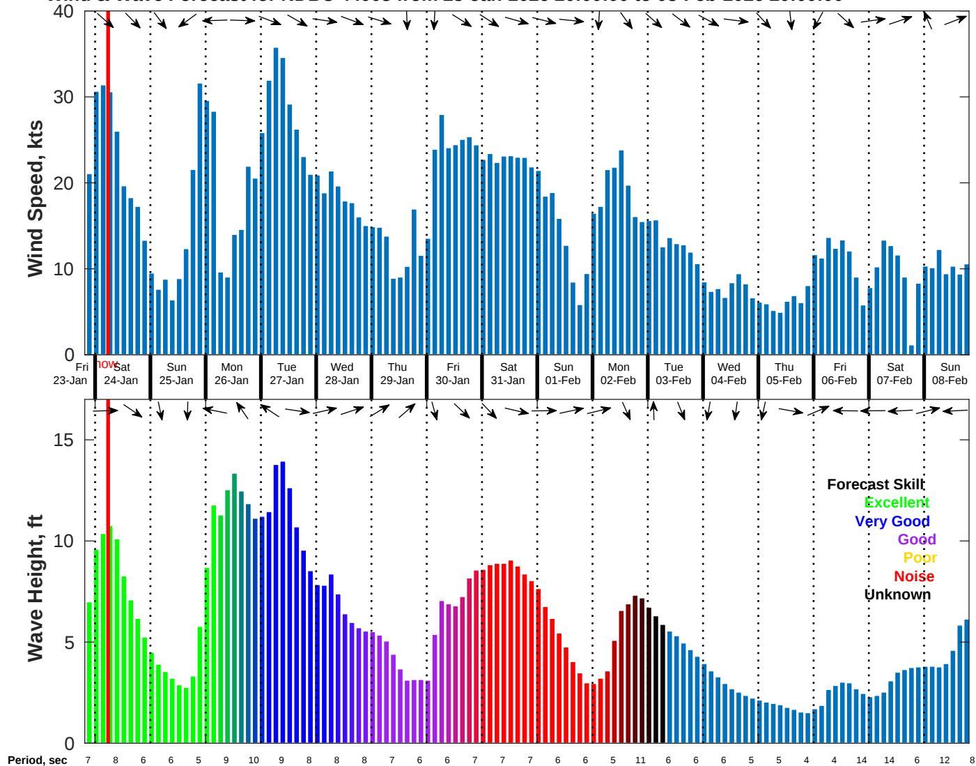
Wind & Wave Forecast for NDBC 44008 from 23-Jan-2026 20:00:00 to 08-Feb-2026 20:00:00
