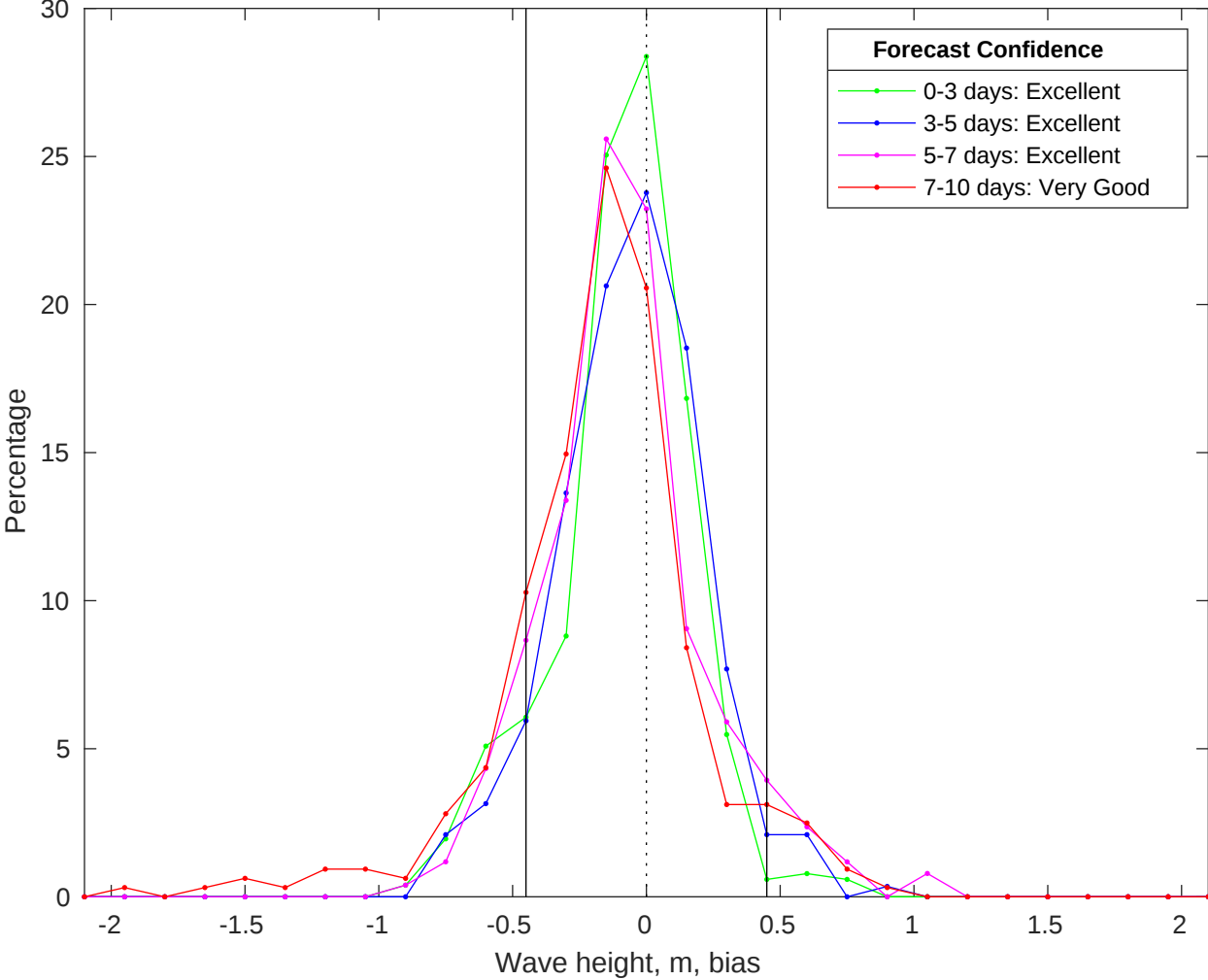
NDBC 46011 vs CMEMS Waves Bias Histogram: 24-Jan-2026
