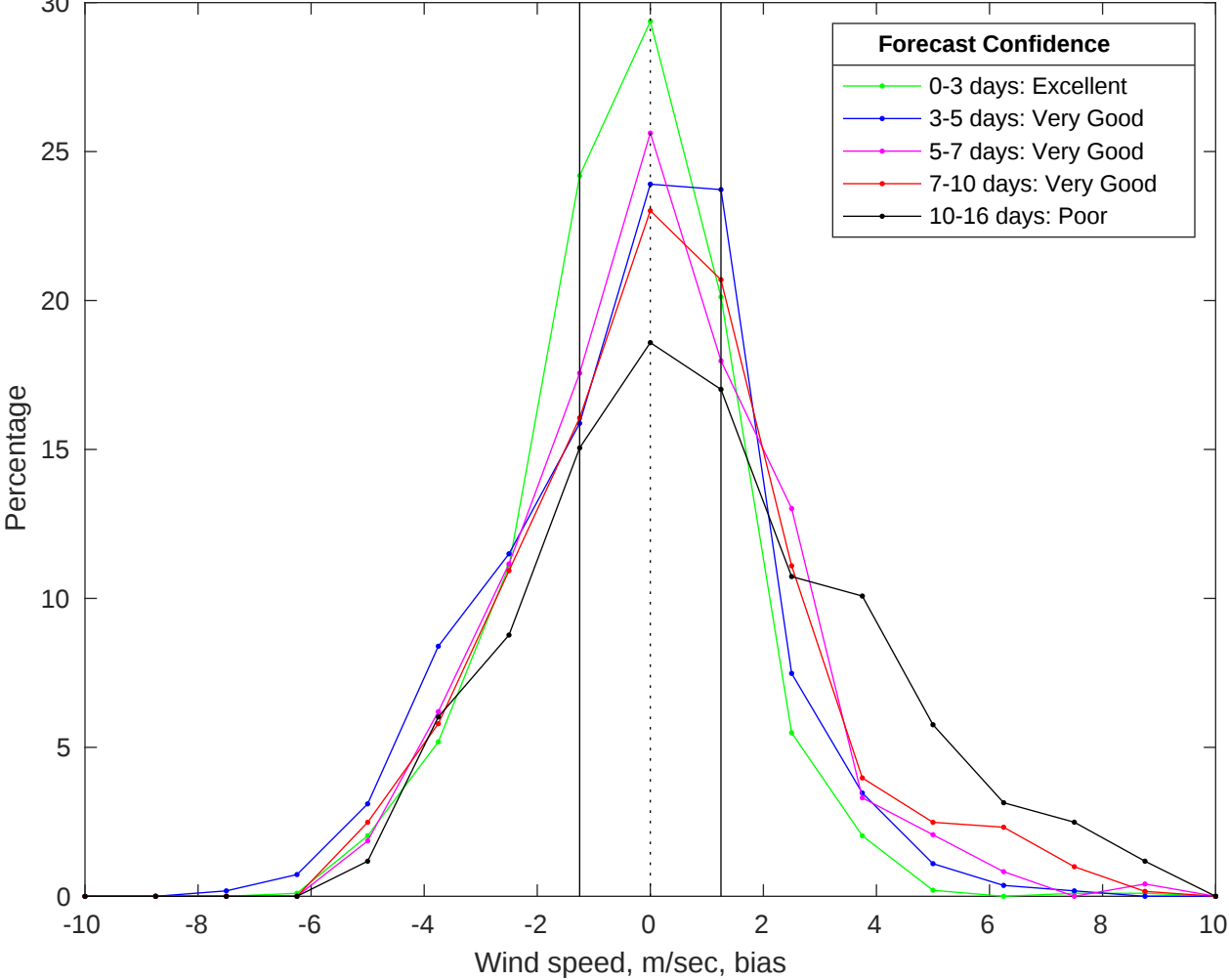
NDBC 46011 vs GFS Winds Bias Histogram: 24-Jan-2026
