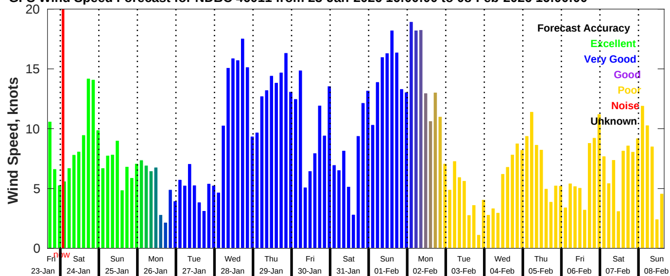
GFS Wind Speed Forecast for NDBC 46011 from 23-Jan-2026 16:00:00 to 08-Feb-2026 16:00:00
