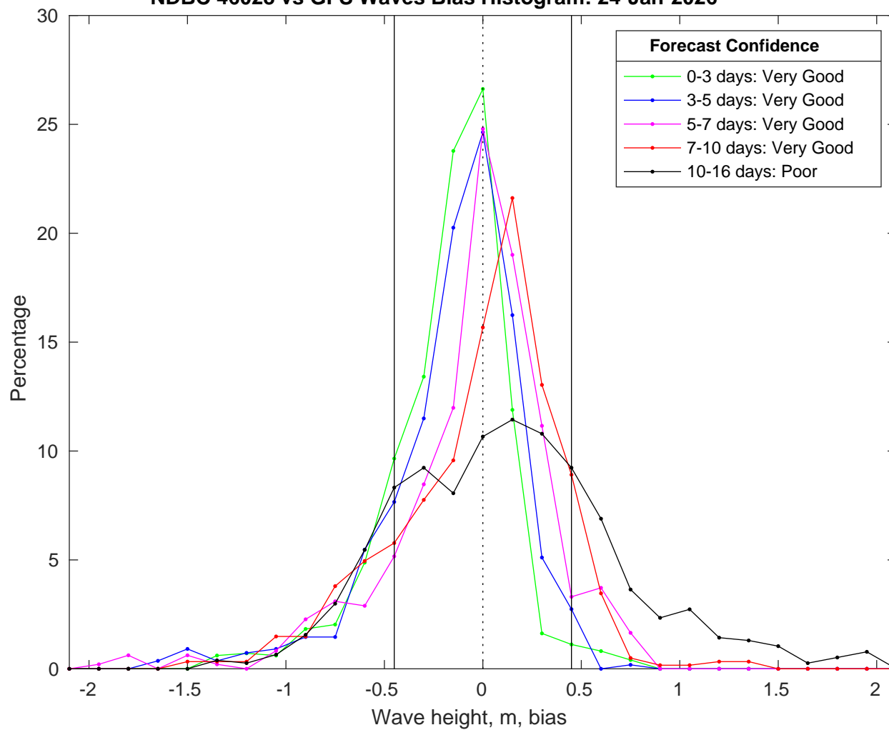
NDBC 46028 vs GFS Waves Bias Histogram: 24-Jan-2026
