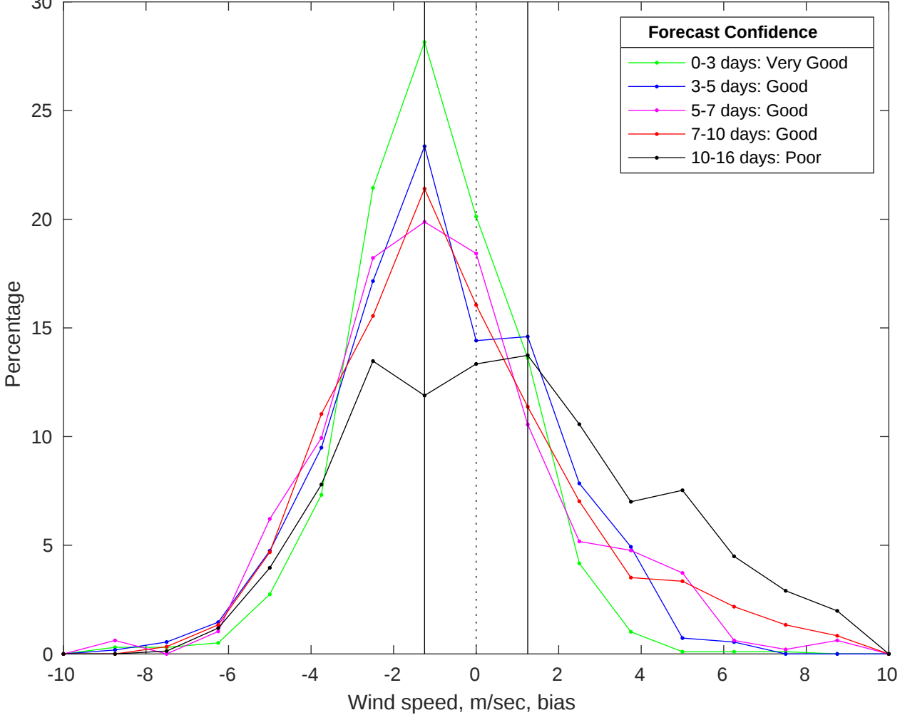
NDBC 46028 vs GFS Winds Bias Histogram: 24-Jan-2026
