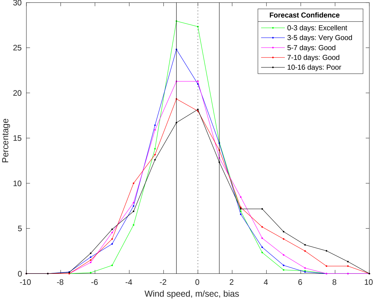
NDBC 46054 vs GFS Winds Bias Histogram: 24-Jan-2026
