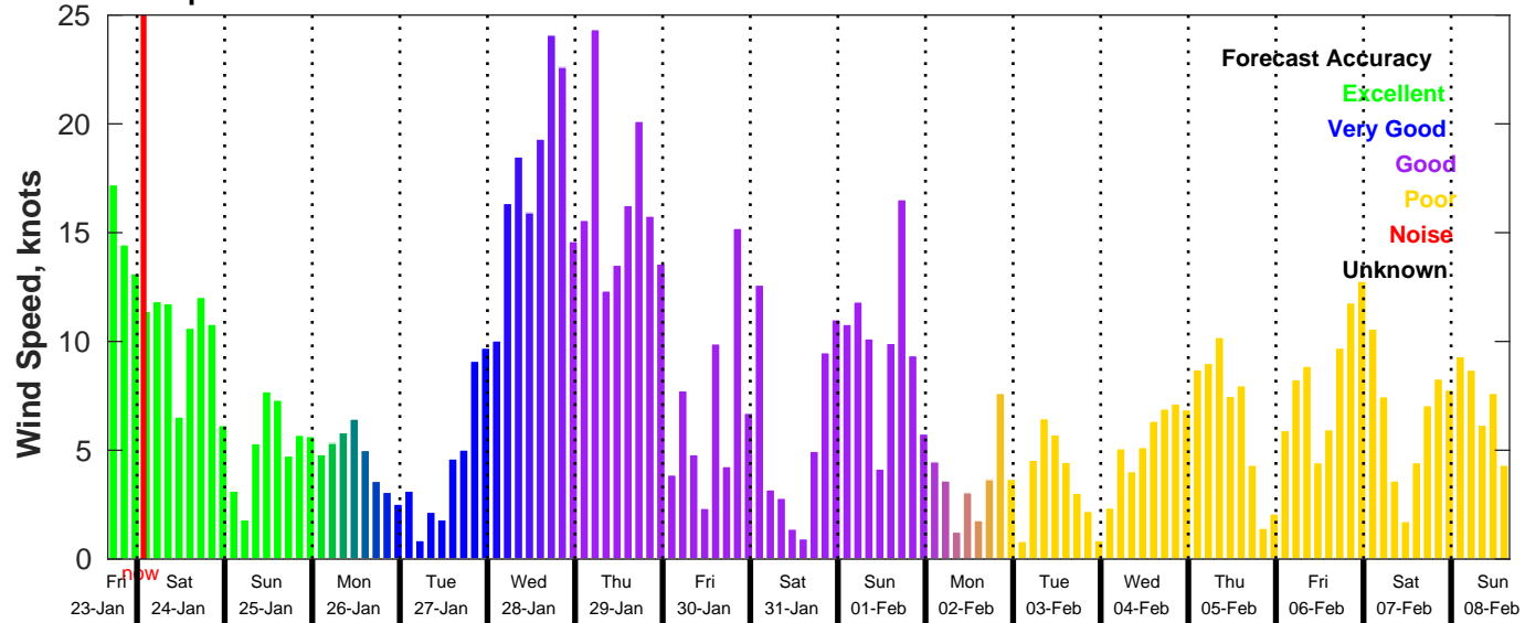
GFS Wind Speed Forecast for NDBC 46054 from 23-Jan-2026 16:00:00 to 08-Feb-2026 16:00:00
