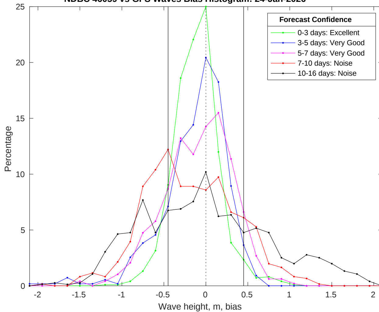
NDBC 46059 vs GFS Waves Bias Histogram: 24-Jan-2026
