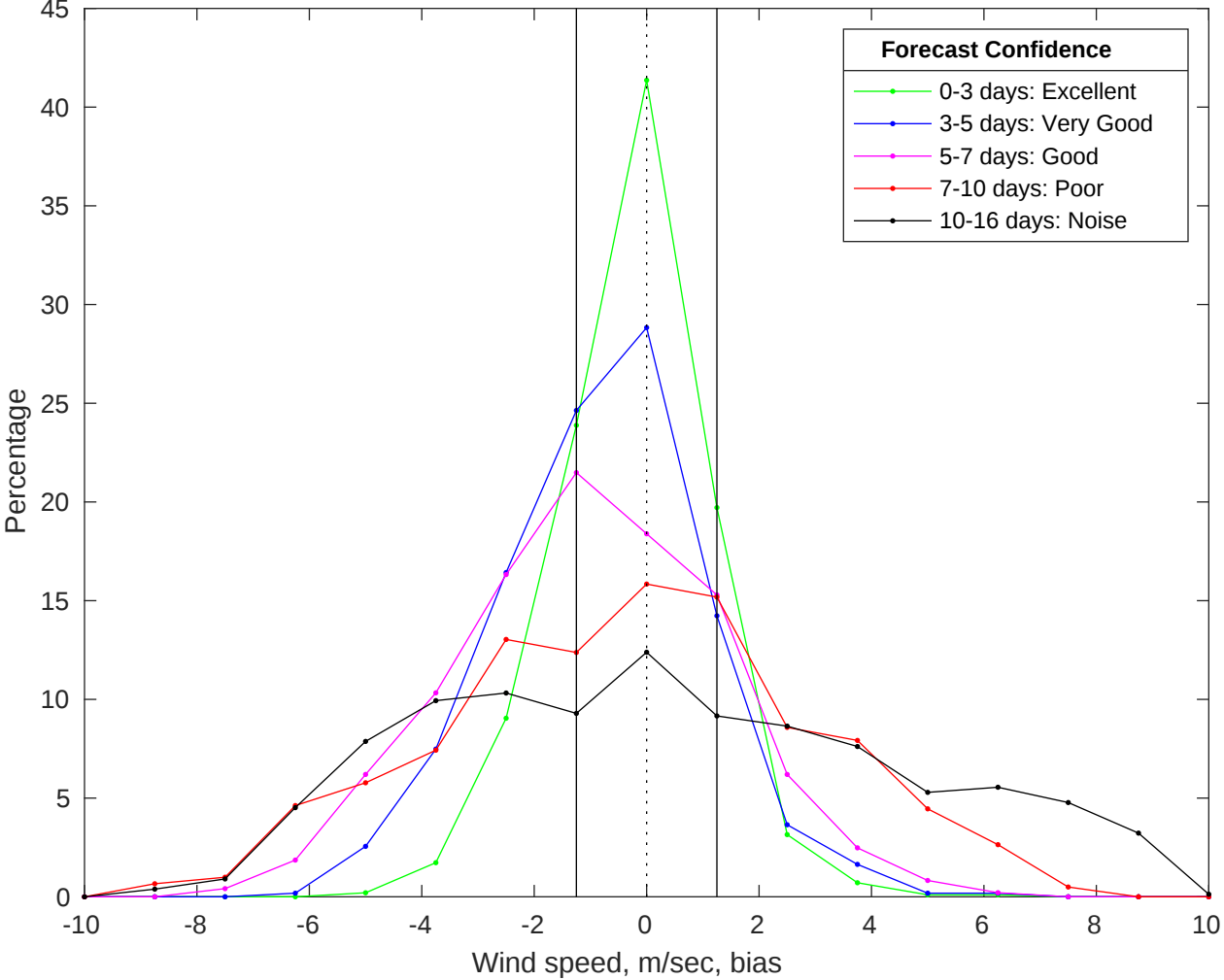
NDBC 46059 vs GFS Winds Bias Histogram: 24-Jan-2026
