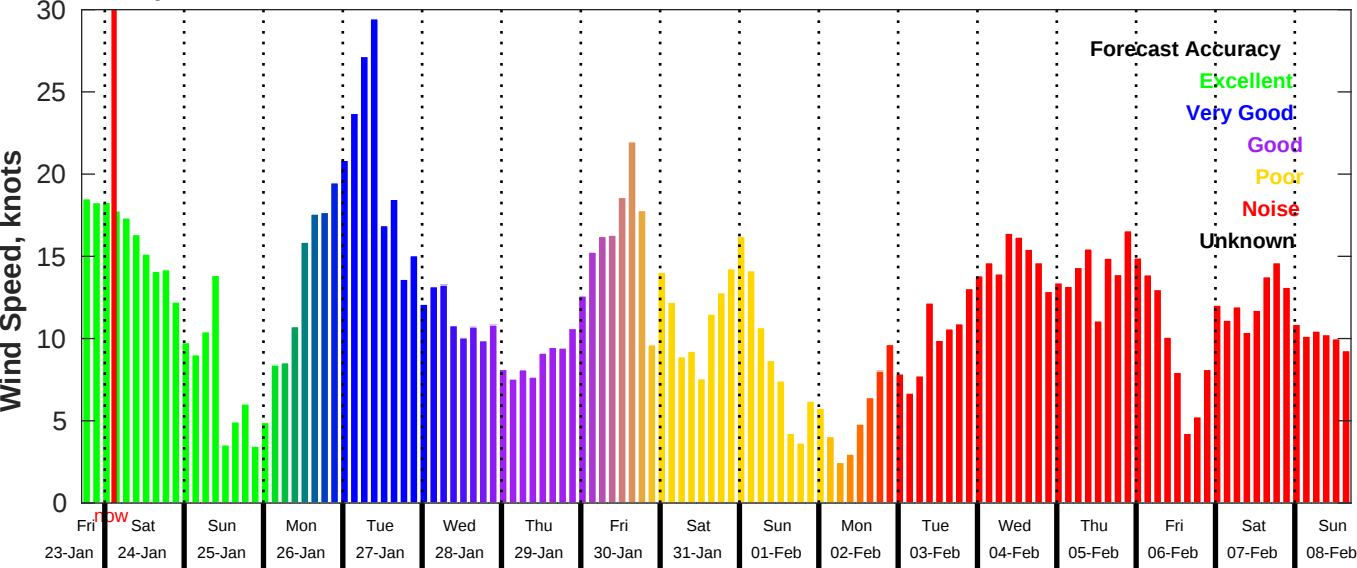
GFS Wind Speed Forecast for NDBC 46059 from 23-Jan-2026 17:00:00 to 08-Feb-2026 17:00:00
