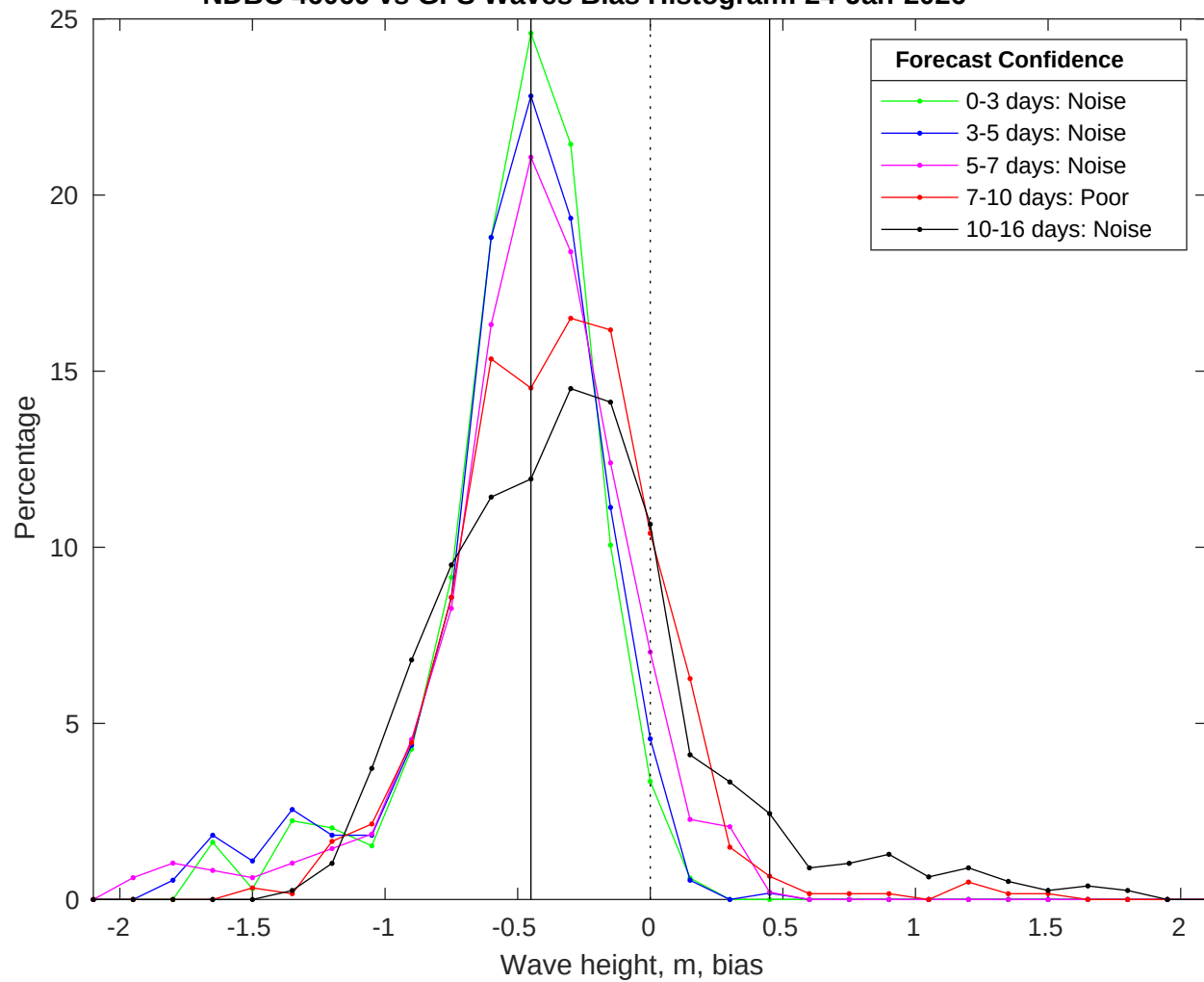
NDBC 46069 vs GFS Waves Bias Histogram: 24-Jan-2026
