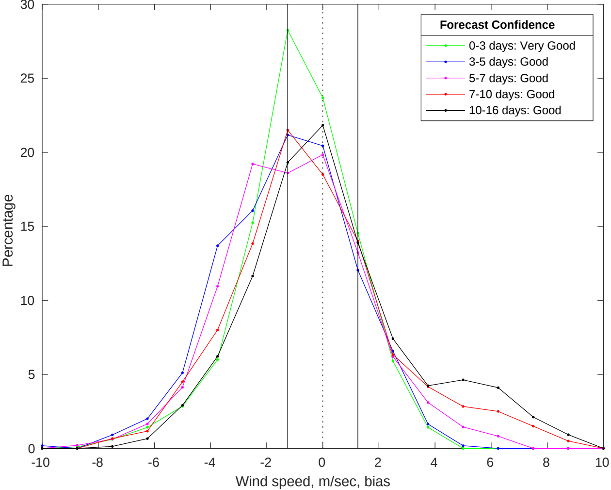
NDBC 46069 vs GFS Winds Bias Histogram: 24-Jan-2026
