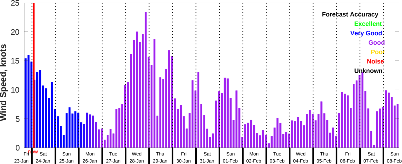
GFS Wind Speed Forecast for NDBC 46069 from 23-Jan-2026 16:00:00 to 08-Feb-2026 16:00:00
