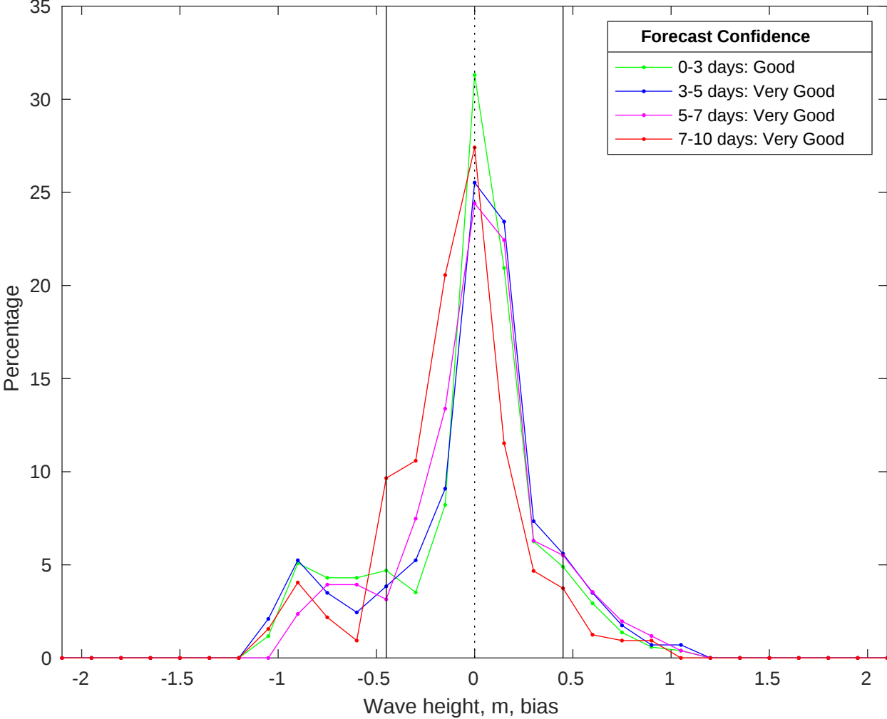
NDBC 46215 vs CMEMS Waves Bias Histogram: 24-Jan-2026
