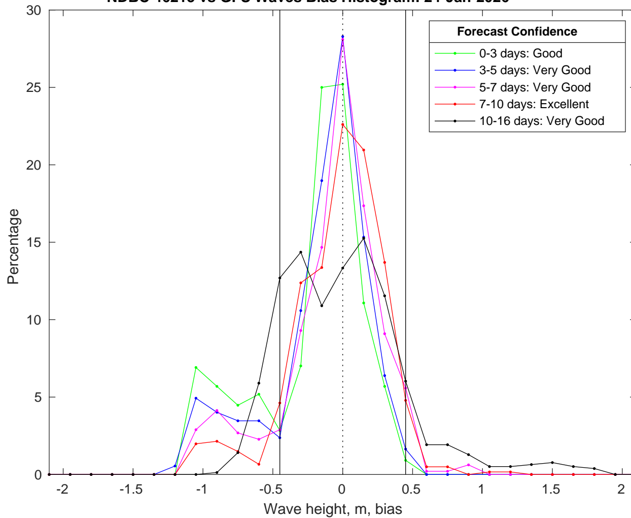
NDBC 46215 vs GFS Waves Bias Histogram: 24-Jan-2026
