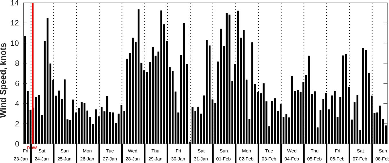
GFS Wind Speed Forecast for NDBC 46215 from 23-Jan-2026 16:00:00 to 08-Feb-2026 16:00:00
