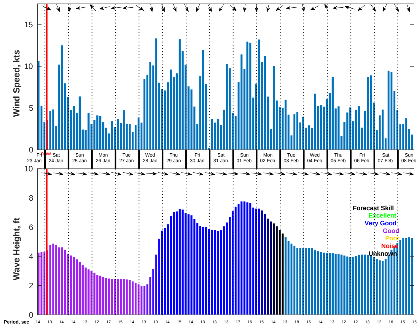
Wind & Wave Forecast for NDBC 46215 from 23-Jan-2026 16:00:00 to 08-Feb-2026 16:00:00
