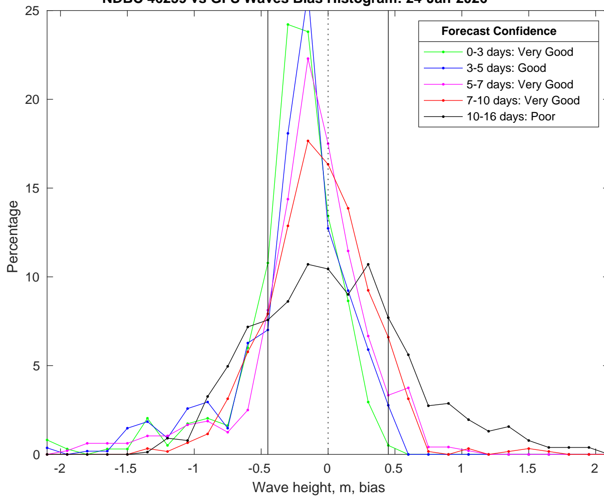
NDBC 46259 vs GFS Waves Bias Histogram: 24-Jan-2026
