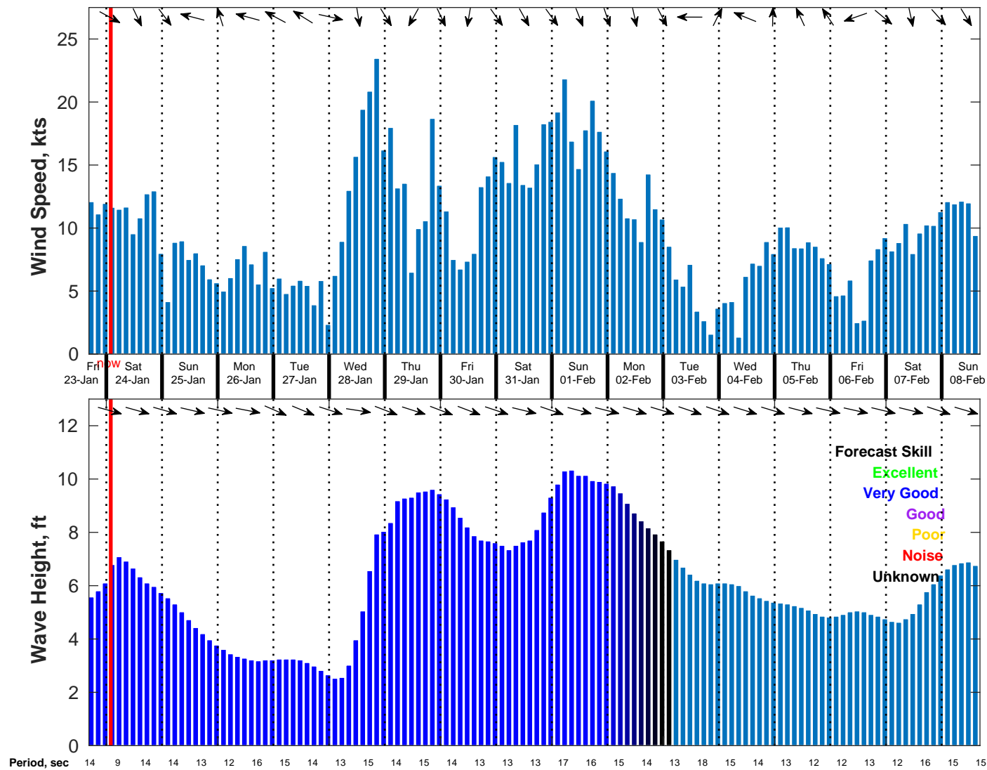
Wind & Wave Forecast for NDBC 46259 from 23-Jan-2026 16:00:00 to 08-Feb-2026 16:00:00
